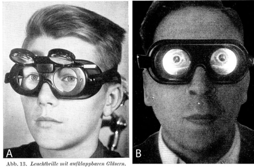
Figure 1 Dr Frenzel's nystagmus goggles. Open (A), closed (B) and illuminated from within. (from Frenzel 5 ).
